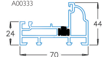
French Door Low Threshold A00333
